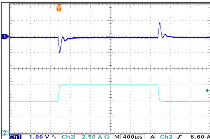
Figure 5: Output voltage response to step-change in load current (50%-75%-50% of I_{out(max)} ; dI/dt = 0.1 A/\mu s ). Load cap: 1 \mu F ceramic capacitor. Ch 1: V_{out} , Ch 2: I_{out} (2.5A/div.)
